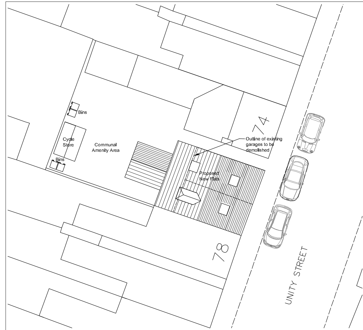
PROPOSED BLOCK AND ROOF PLAN 1:200
